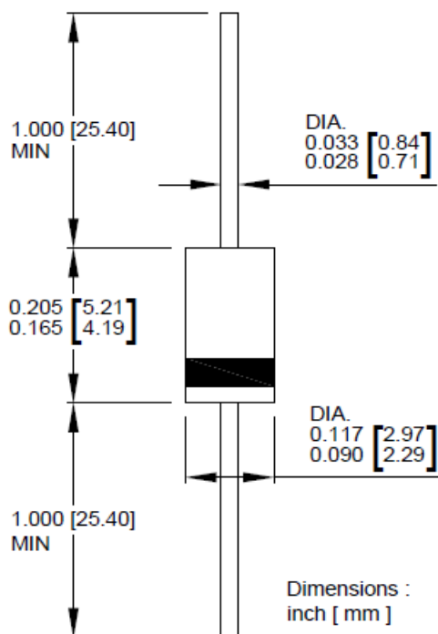
DO-41
